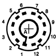
1 pole 12 way 30° Throw
