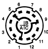
3 pole 4 way 30° Throw
