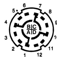
4 pole 3 way 30° Throw
