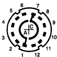
2 pole 6 way 30° Throw
