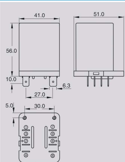
Panel Mountable
