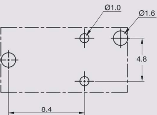
1 Form A
