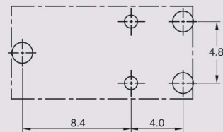
1 Form C
