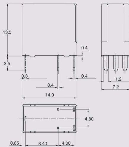
1 Form C
