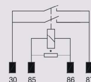
1 Form A
